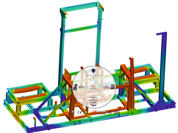
Deflection on Skid Structure during transportation
