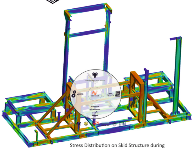
Stress Distribution on Skid Structure during transportation
