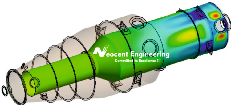
FEA Stress Analysis post processing under ASME Div 2.
